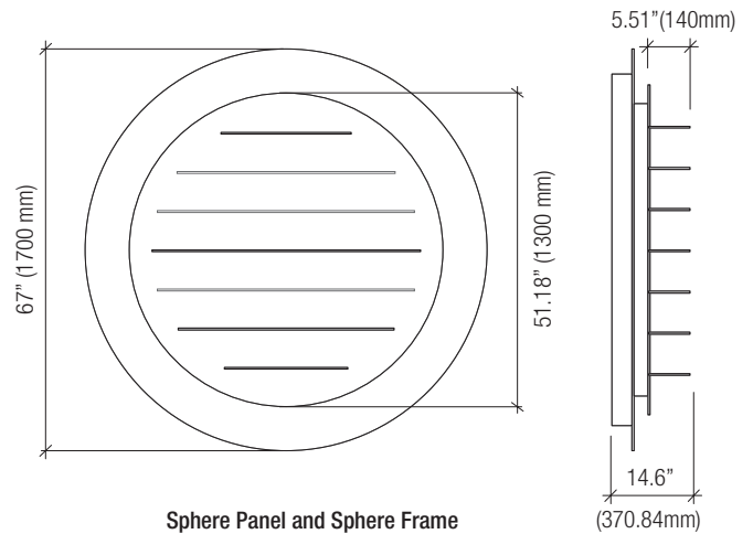
Sphere Panel and Sphere Frame
