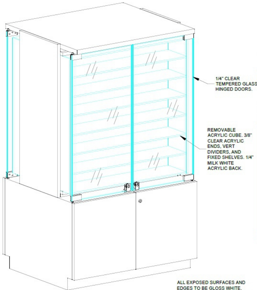
FRONT ISOMETRIC
