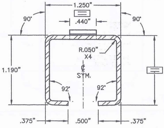
Duct-O-Wire
