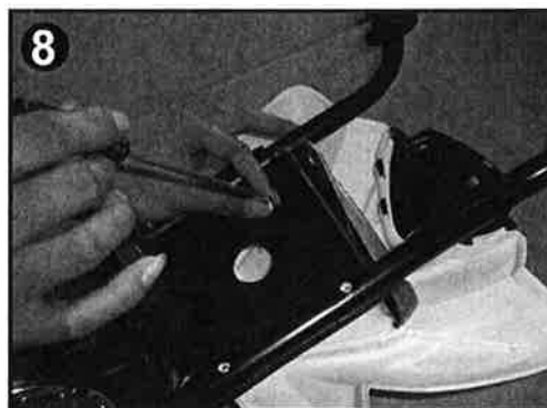
Fasten the screws (3.5x12) x4 pcs on the head rack.
