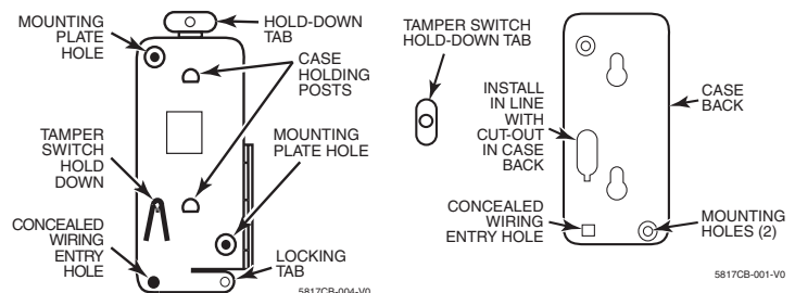
Figure 2. Case Back
