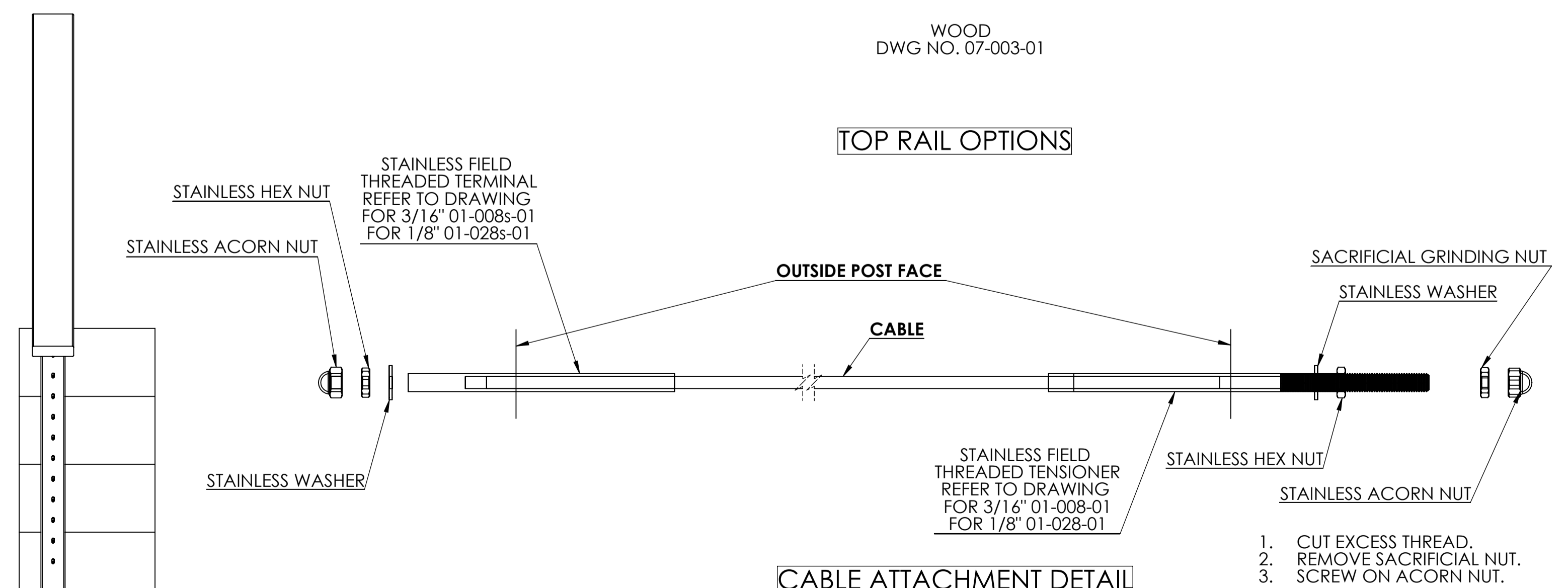
CABLE ATTACHMENT DETAIL
