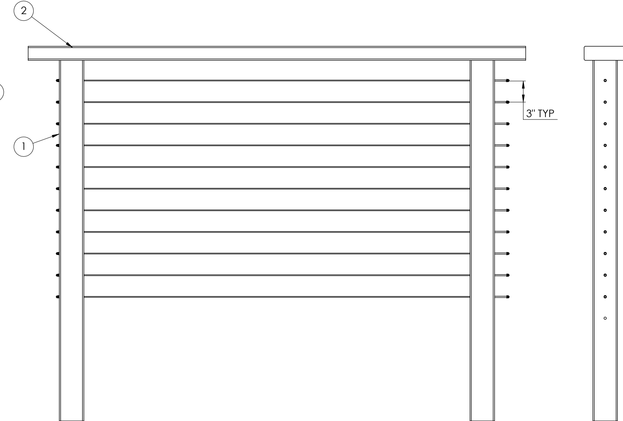
LEVEL 36" STANDARD GUARD RAILING
