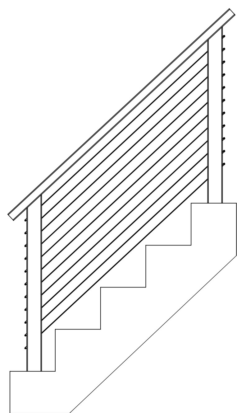
STAIRS 36" STANDARD GUARD RAILING
