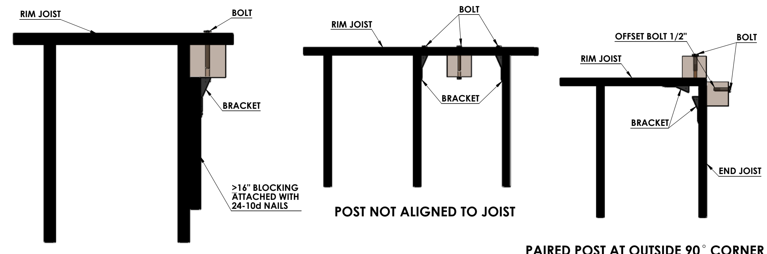
PAIRED POST AT OUTSIDE 90° CORNER
