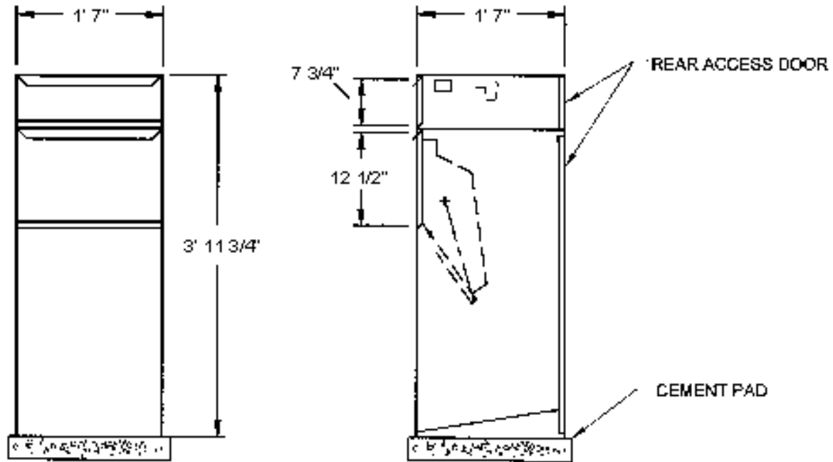
Curbside Vault with Locking Letterbox and Outgoing Compartment Model Number DVCS0015
