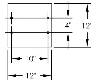
PEDESTAL BASE BOLT PATTERN
