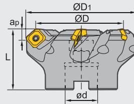
C type of mounting
