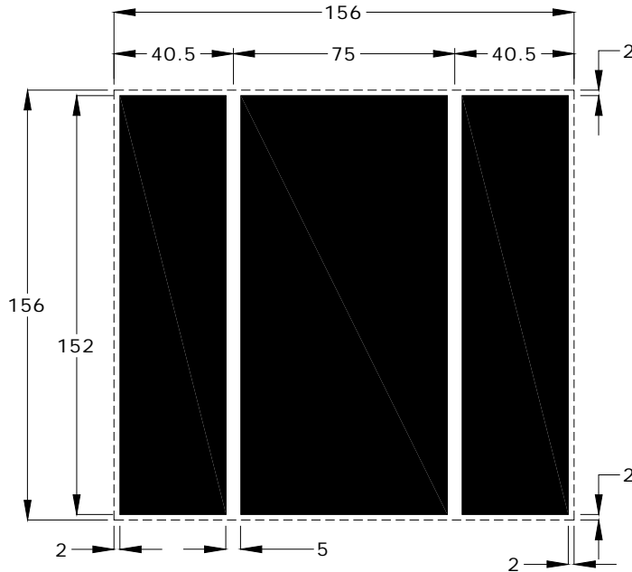
SPI-C156-xxxM2 Product Series - Solar Cell Back
