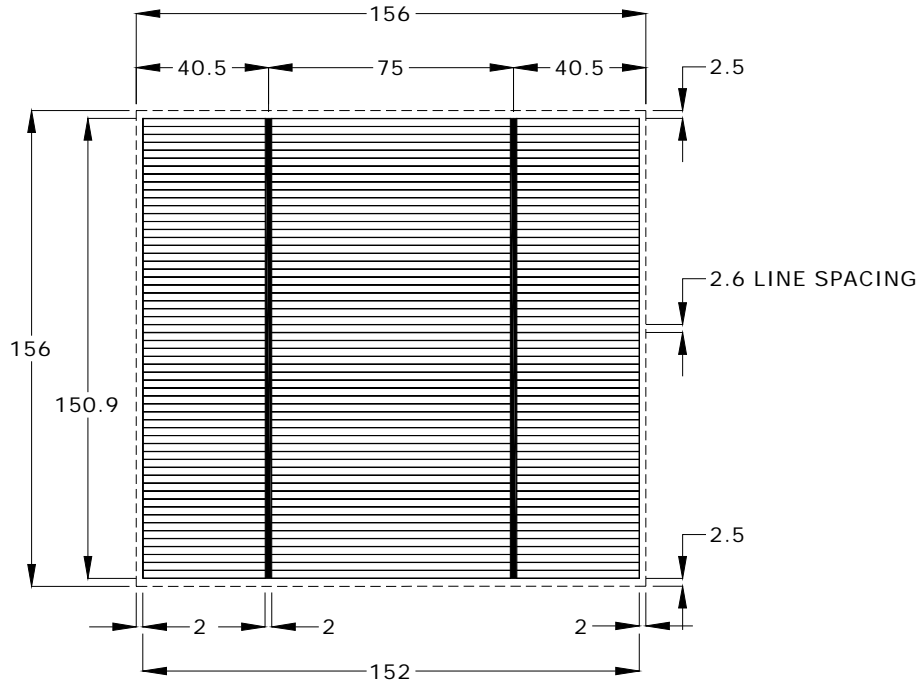
SPI-C156-xxxM2 Product Series - Solar Cell Front
