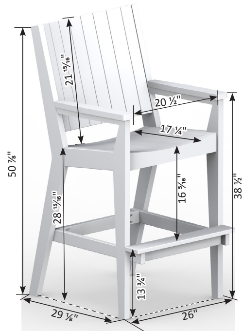
Mayhew Chat XT Chair
