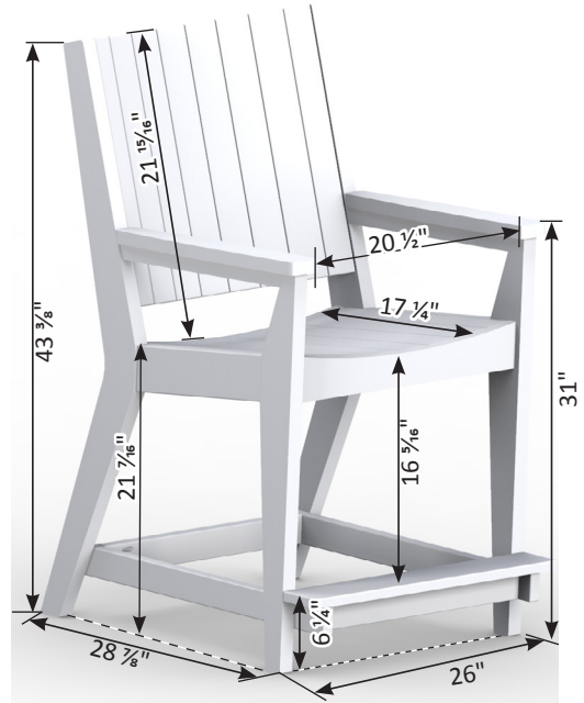
Mayhew Chat Counter Chair
