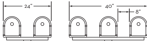
FAIRFIELD WITH STANDARD POST
