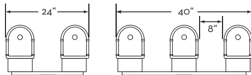
FAIRFIELD WITH STANDARD POST
