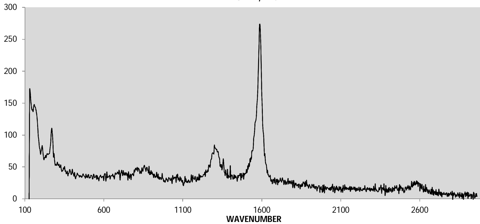
Raman, 785nm PD1.5L1-5 SWNT, 20120628 NANOLAB, INC
